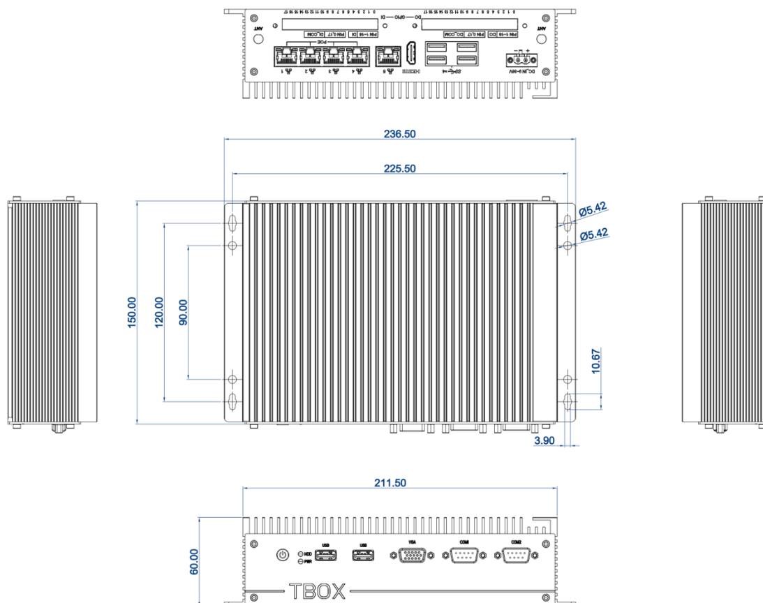
DIMENSIONAL DRAWING:TBOX-3TX0/3DX0
