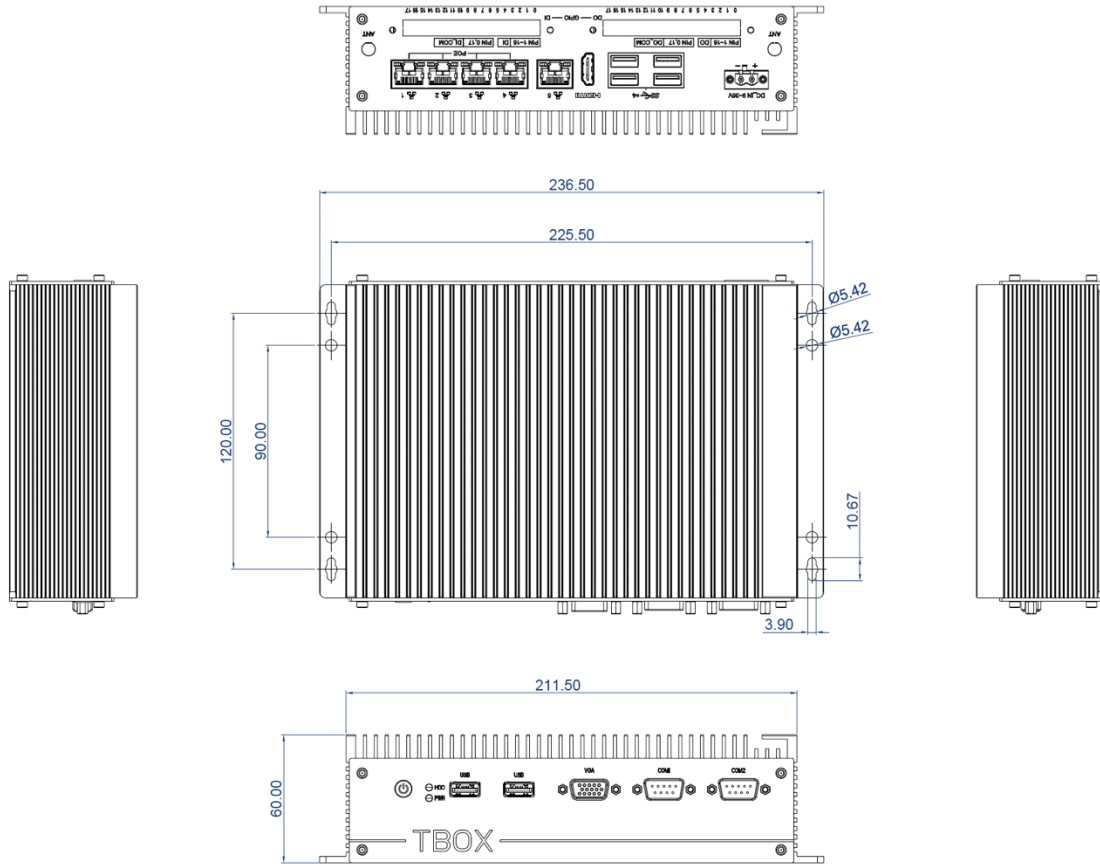
DIMENSIONAL DRAWING:TBOX-3TX0
