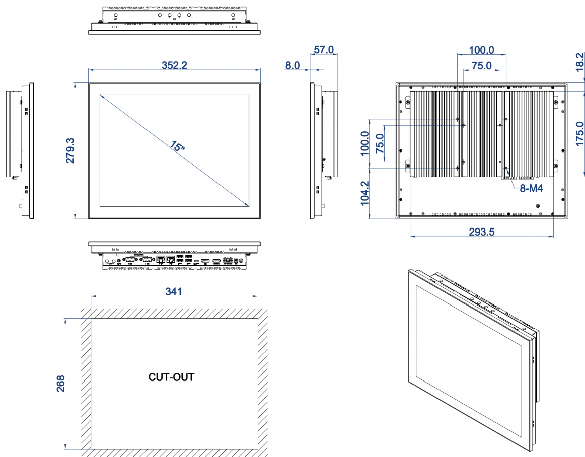
DIMENSIONAL DRAWING:TPC-DCT150
